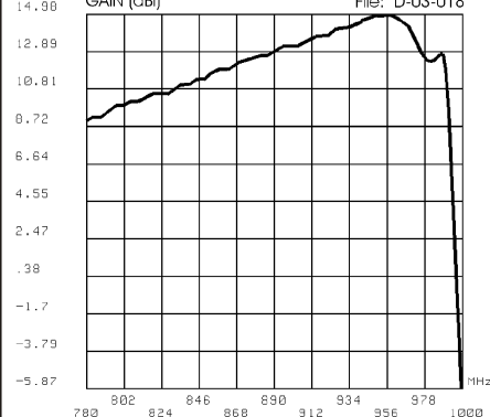
TYPICAL GAIN DIAGRAM vs FREQUENCY
