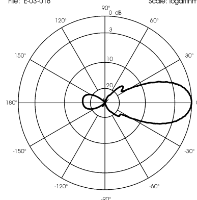
TYPICAL RADIATION PATTERN in H-plane at 890 MHz
